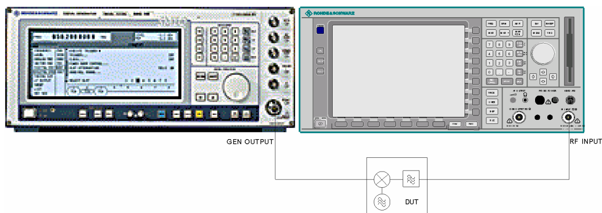
Fig. 4.35 Test setup for frequency-converting measurements
