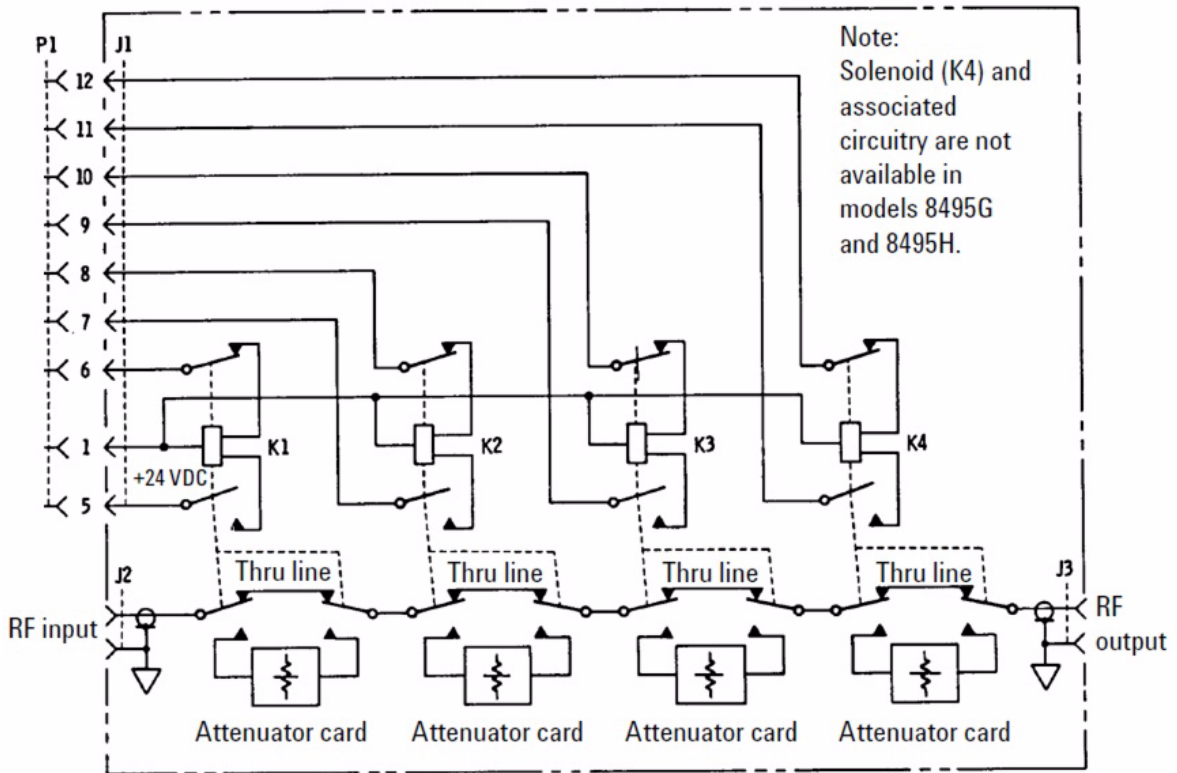
Figure 1 Typical Four-Section Attenuator Schematic Diagram
